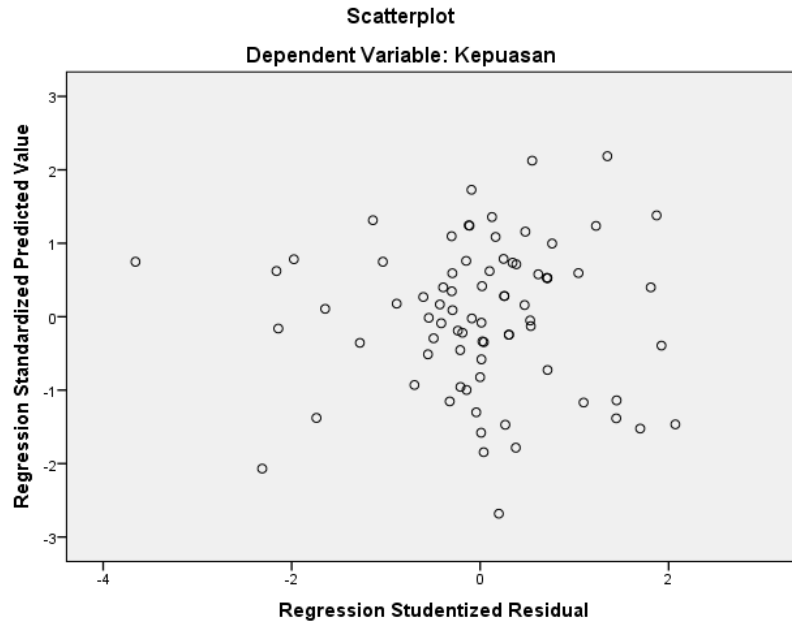
Figure 3: Scatterplot Heteroscedasticity Test Results
