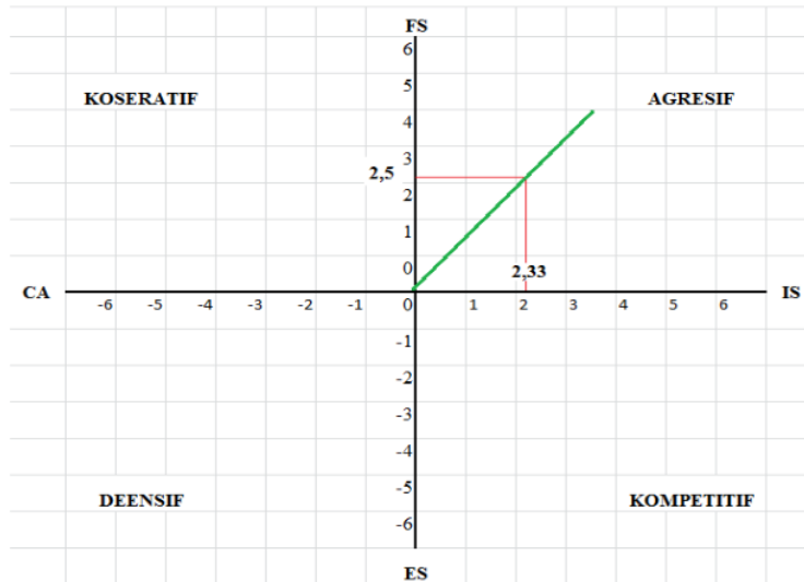
Gambar 1. Matriks Space
