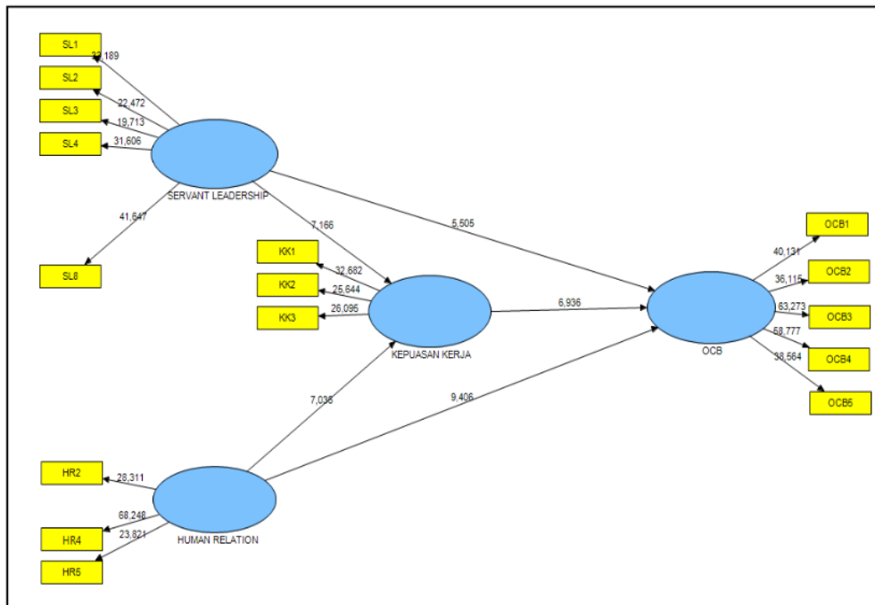
Figure 2: Path analysis Source: Results of SmartPLS data processing, Year 2021
