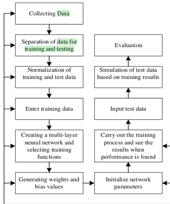
FIGURE 1. General Research Method Flowchart
