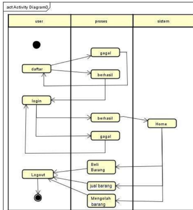
Gambar6.3 Activity Diagram User
