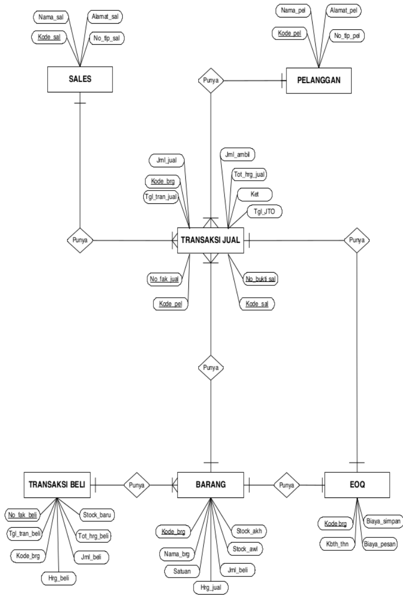
Gambar 6.5. Entity Relationship Diagram (ERD)
