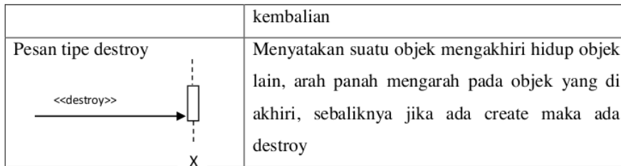
Gambar 1.4 Simbol Sequence diagram
