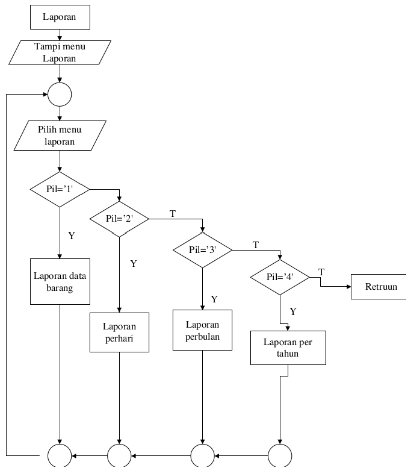
Gambar 1.33 Flowchart Laporan
