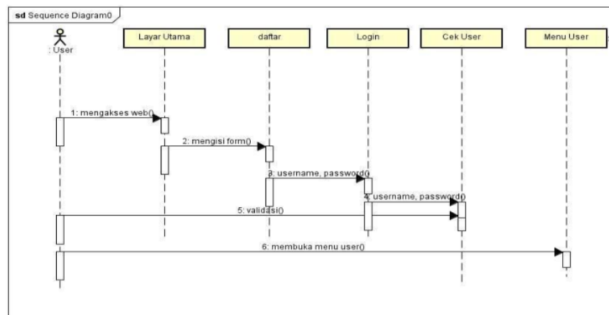
Gambar6.5 SequenceDiagram User
