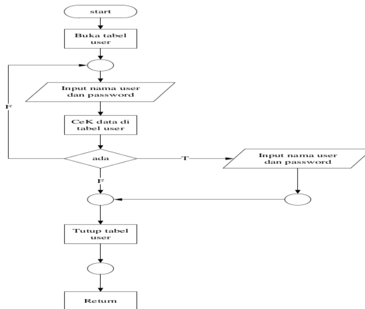
Gambar 1.30 Flowchart Login
