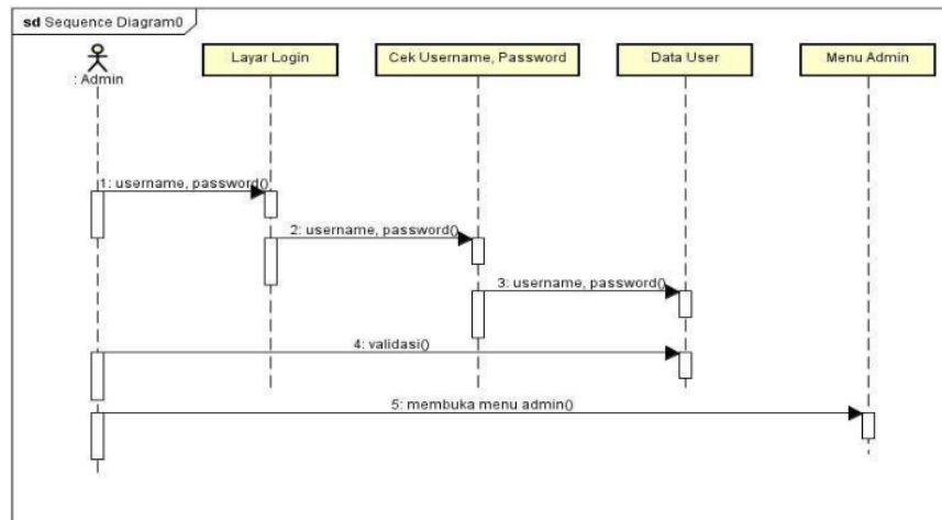
Gambar6.4 SequenceDiagram Admin
