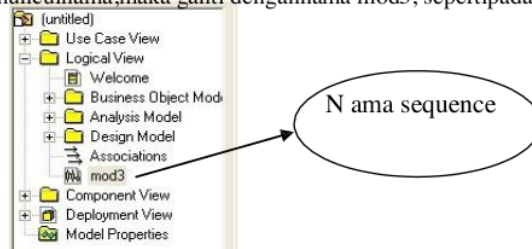
Gambar4.3 Nama sequence
