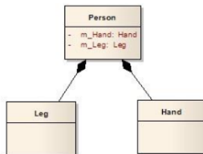
Gambar 3.7 Contoh composition
