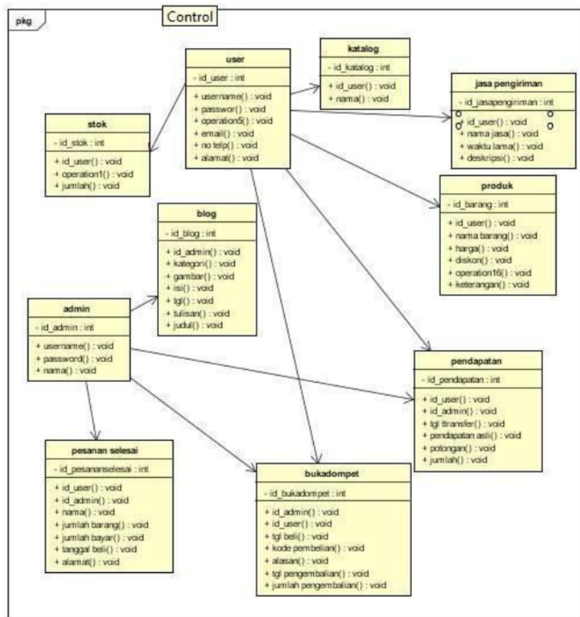
Gambar6.6 ClassDiagram SistemInformasiMarketplace
