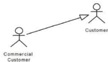
Gambar2.1Actor
