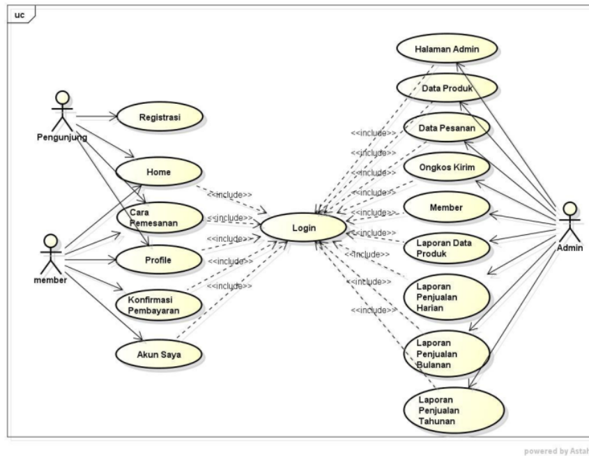
Gambar 1.5 Use Case Diagram
