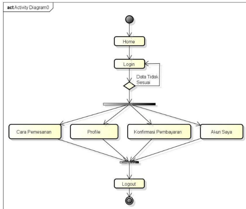
Gambar 1.8 Activity Diagram Kustomer
