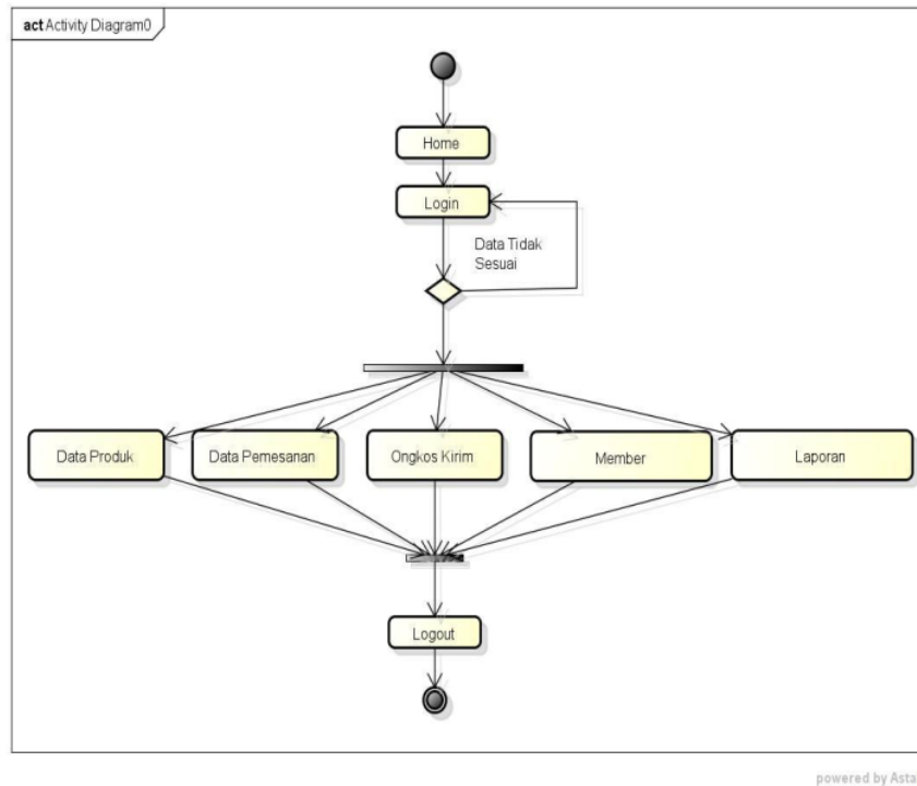
Gambar 1.7 Activity Diagram Admin
