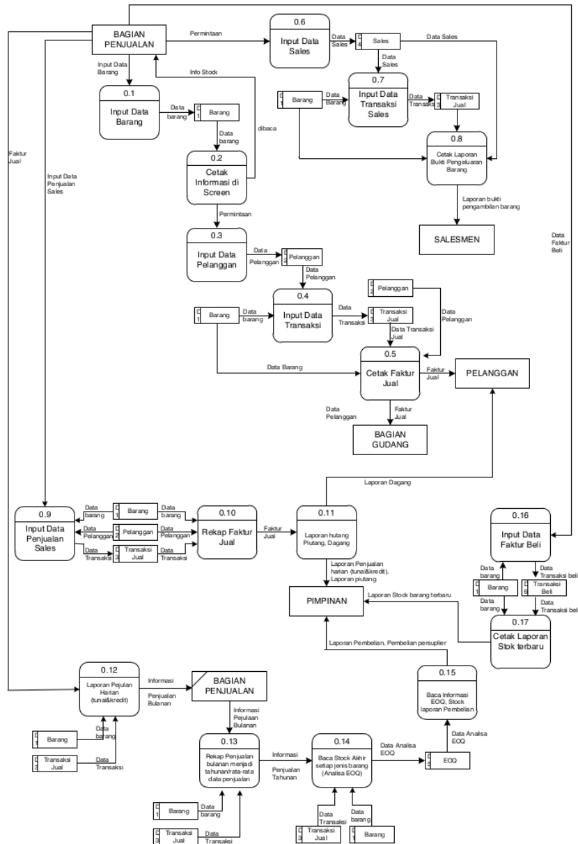
Gambar 6.4. Data Flow Diagram (DFD) Level 0
