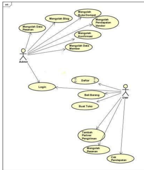
Gambar 6.1 Use Case Sistem Informasi Marketplace
