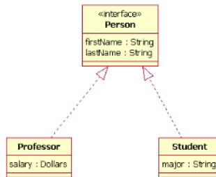
Gambar3.9Contohrealization
