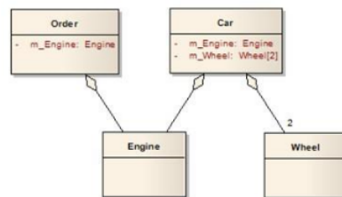
Gambar 3.6 Contoh aggregation
