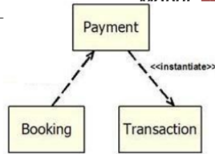
Gambar3.8Contohdependency
