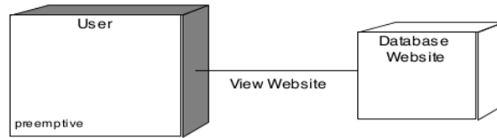
Gambar 1.13 Deployment Diagram
