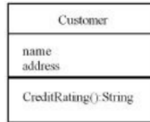
Gambar 3.1 Class
