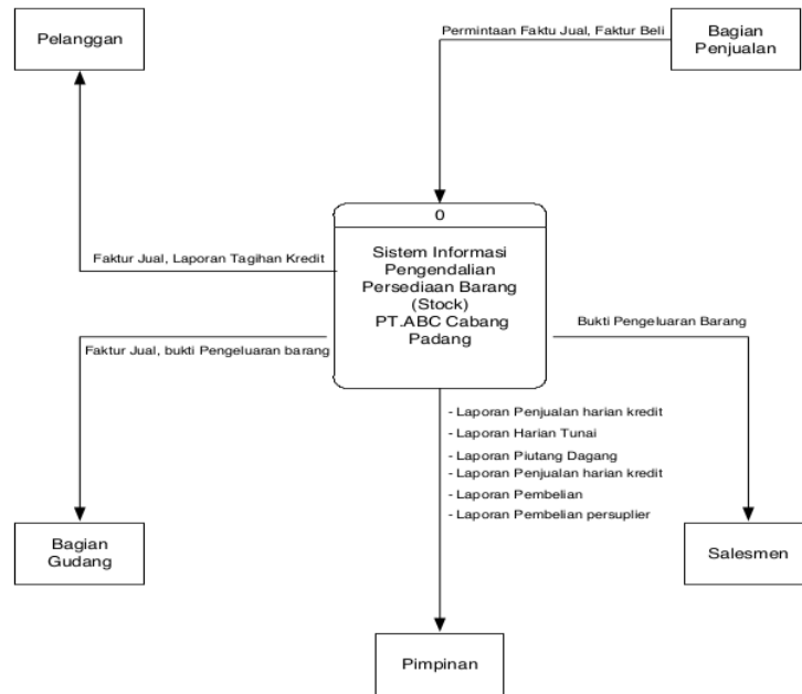
Gambar 6.3. Context Diagram
