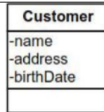
Gambar3.2Atributdari ClassDiagram
