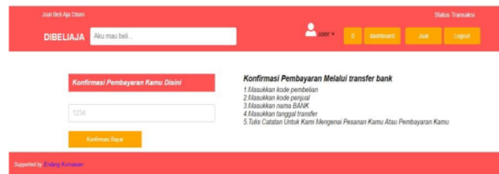
Gambar6.18
