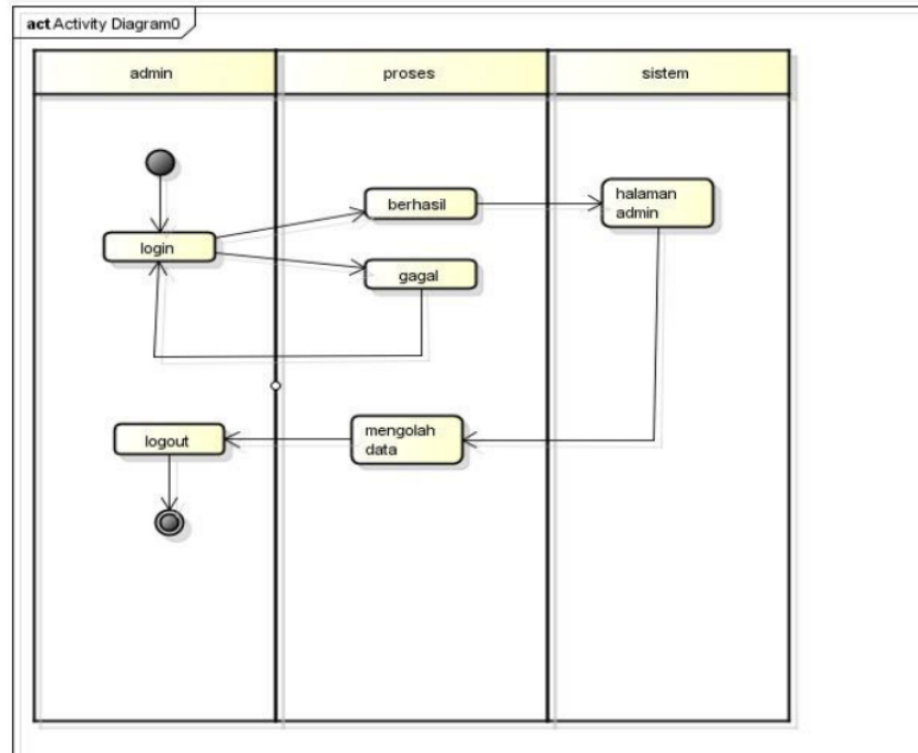
Gambar 6.2 Activity Diagram admin
