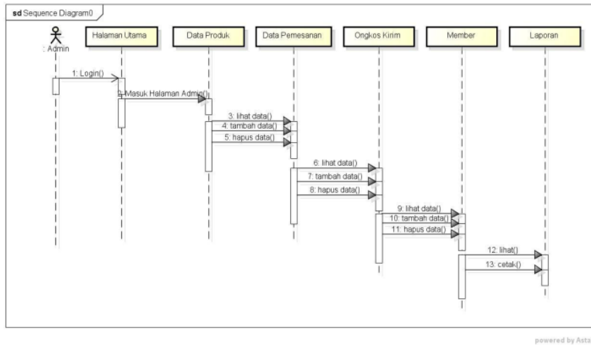
Gambar 1.9 Sequence Diagram Admin Login
