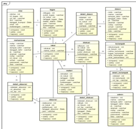
Gambar 4.10. Class Diagram
