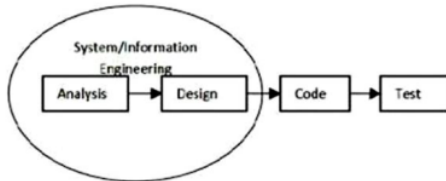
Figure 1. Waterfall Model
