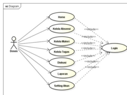
Figure 2. Use Case
