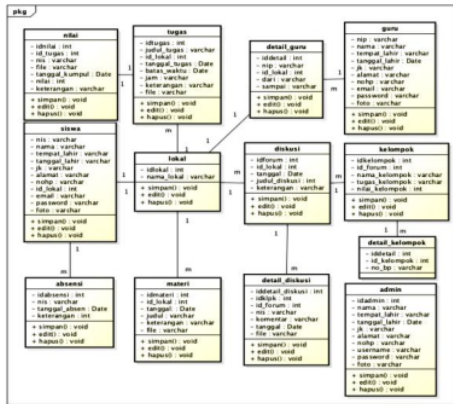
Figure 3. Class Diagram
