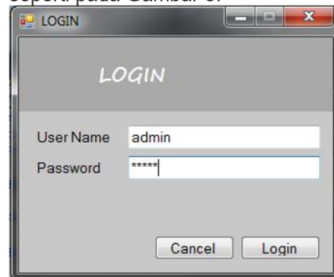
Gambar 8. Login User
