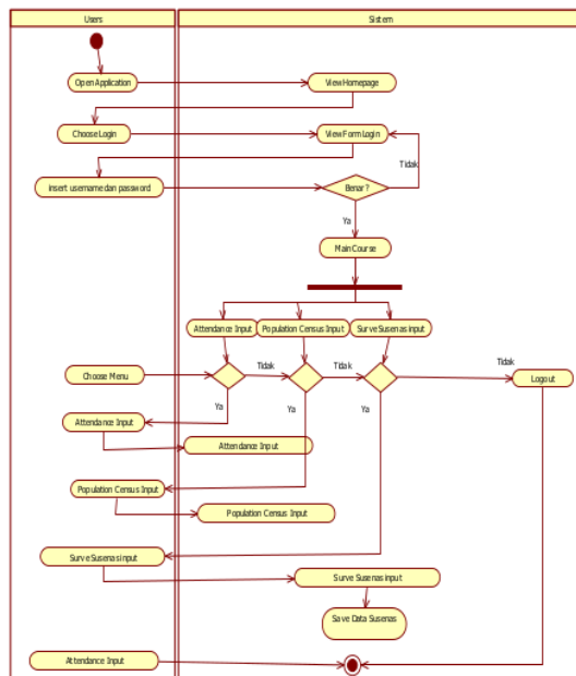
Fig. 5 Activity Diagram
