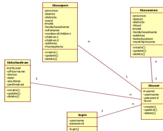
Fig. 4 Class Diagram
