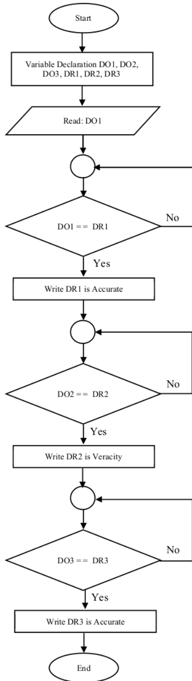
Fig. 6 The Flowchart of Proposed Algorithm
