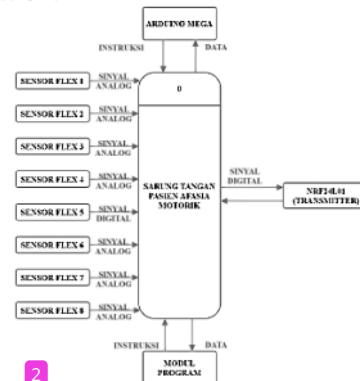
Figure 2. Context Diagram (gloves)
