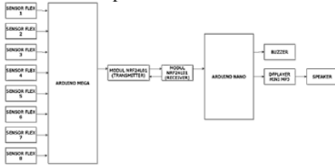
Figure 5. Block Diagram
