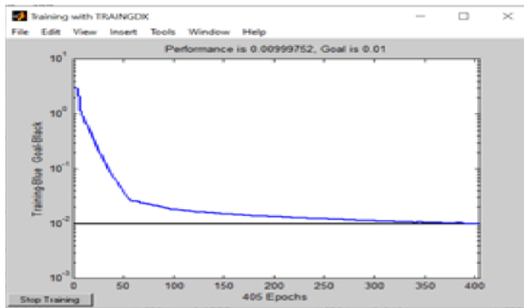
Figure 4. Prediction Results Graph
