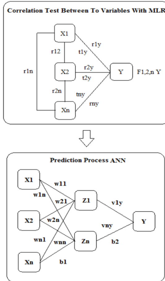
Figure 2. Design Prediction Model
