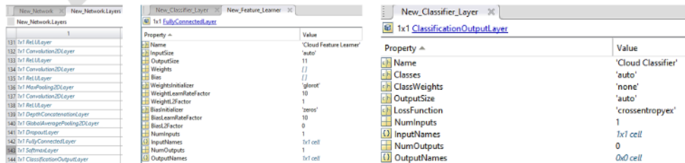
FIGURE 3. Modify the GoogleNet architecture layer
