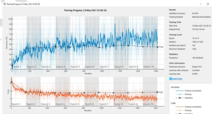
FIGURE 6. The training process of the GoogleNet architecture
