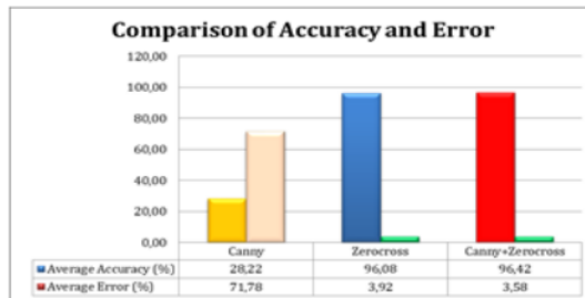
Fig. 5 Comparison Results of 3 Methods (Precision and Error)
