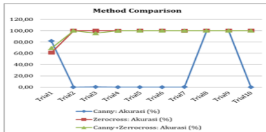
Fig. 4 Comparison Graph of 3 Methods (10 Trials)
