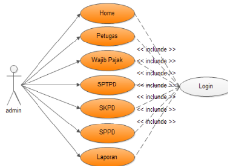
Gambar 4.1 Use case Diagram
