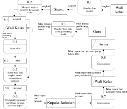
Gambar 3. Data Flow Diagram (DFD)
