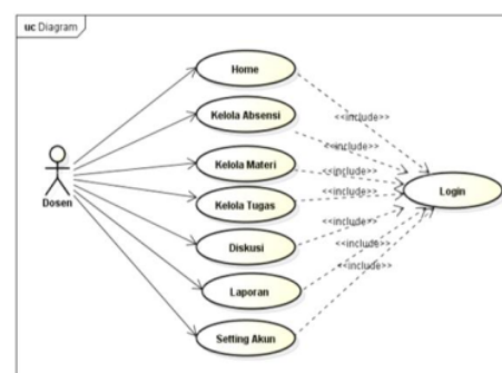
Figure 2. Use Case
