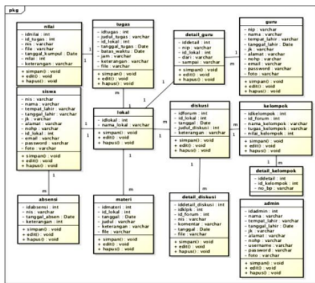
Figure 3. Class Diagram
