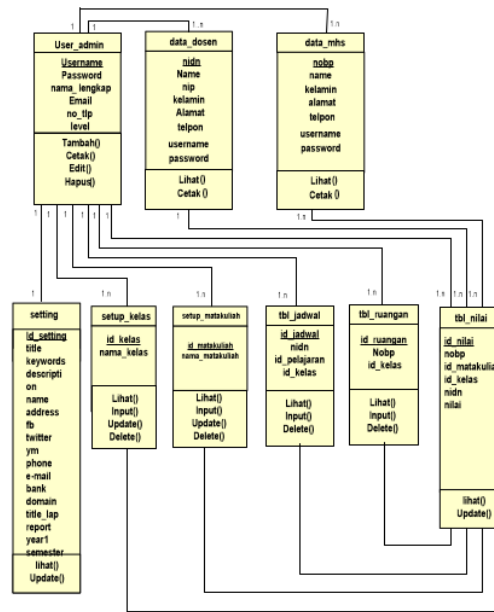
Fig. 4. Class Diagram
