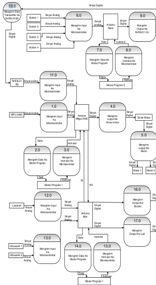
Gambar 3. Data Flow Diagram
