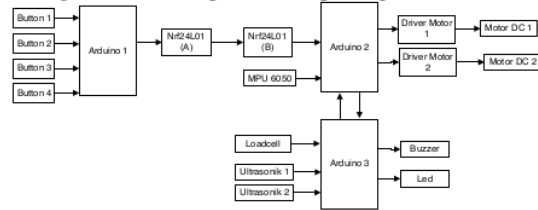
Gambar 4. Blok Diagram
