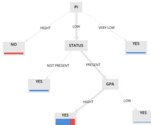
Fig. 6. Decision Tree Prediction Method
