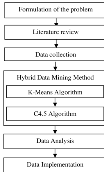
Fig. 1. Research Framework
