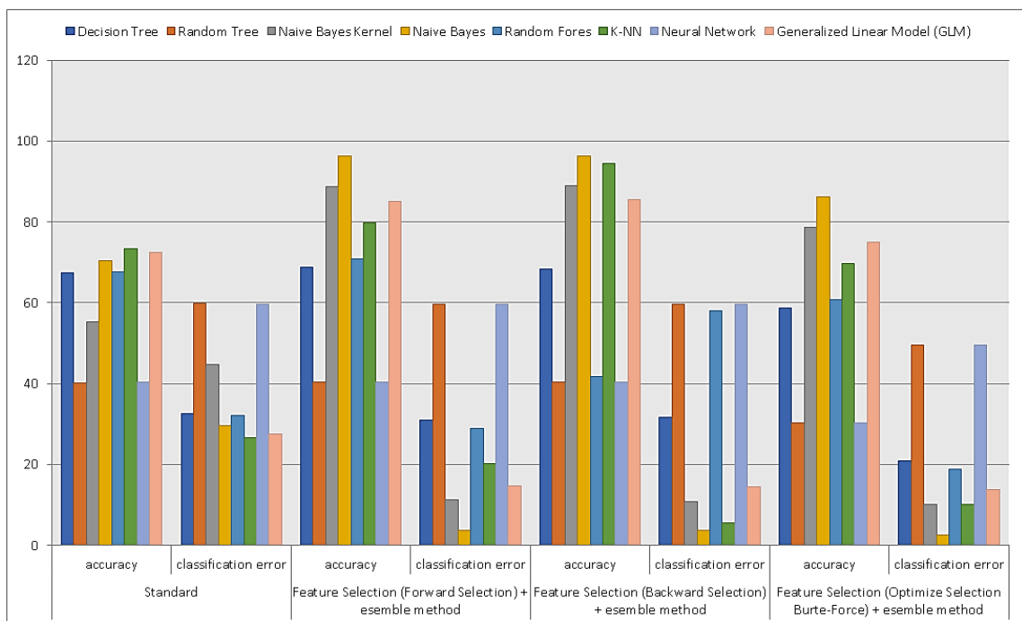
Figure 2. The graphic results summarize the standard classification method and the optimized classification method (accuracy and classification error)
