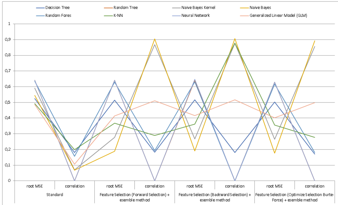
Figure 3. The graphic results summarize the standard classification method and the optimized classification method (root MSE and correlation)
